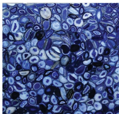
Blue Agate
