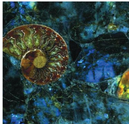
Labradorite
