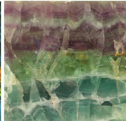
Fluorite
